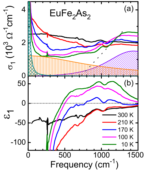
FIG. 6. (Color online) Low-frequency optical properties (up to 1500 \text{ cm}^{-1} ) of \text{EuFe}_2\text{As}_2 at various temperatures for E\parallel ab . (a) The optical conductivity can be decomposed in two Drude-type contributions (olive pattern and orange shaded), and an oscillator to mimic the SDW gap (violet shaded), as depicted for the 10 K data for instance. (b) The frequency dependence of the dielectric constant exhibits a zero crossing ( d\epsilon_1/d\omega > 0 ) as low as 500 \text{ cm}^{-1} .
